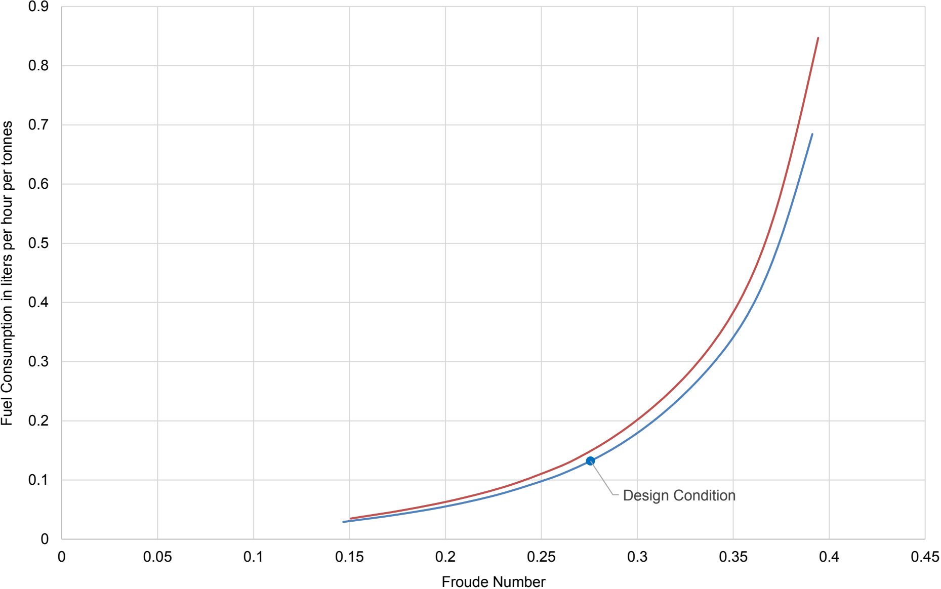
Specific Fuel Consumption vs. Froude Number
